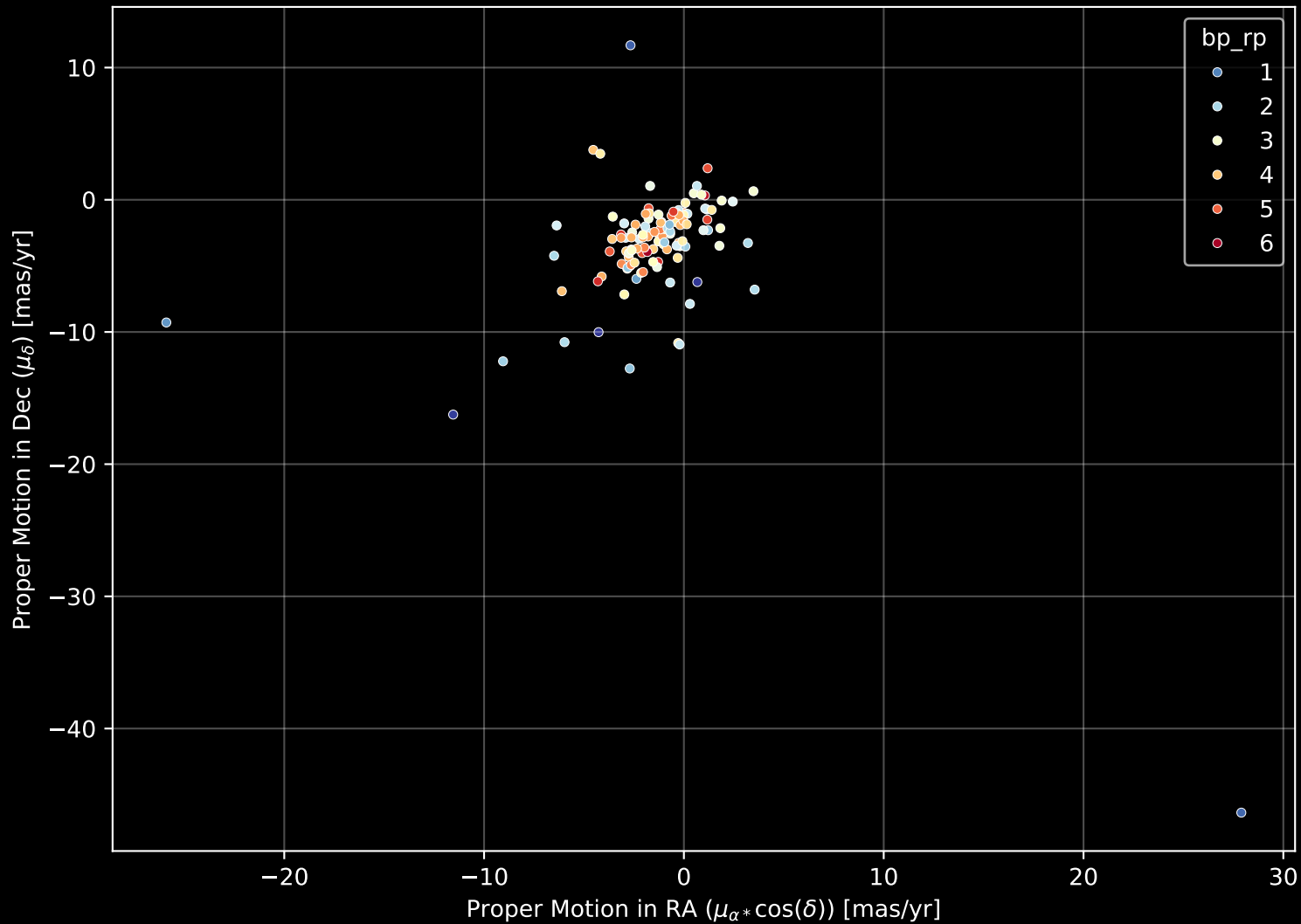
APOGEE DR17 Field: [345+00] Proper Motion Diagram (n= 120)
