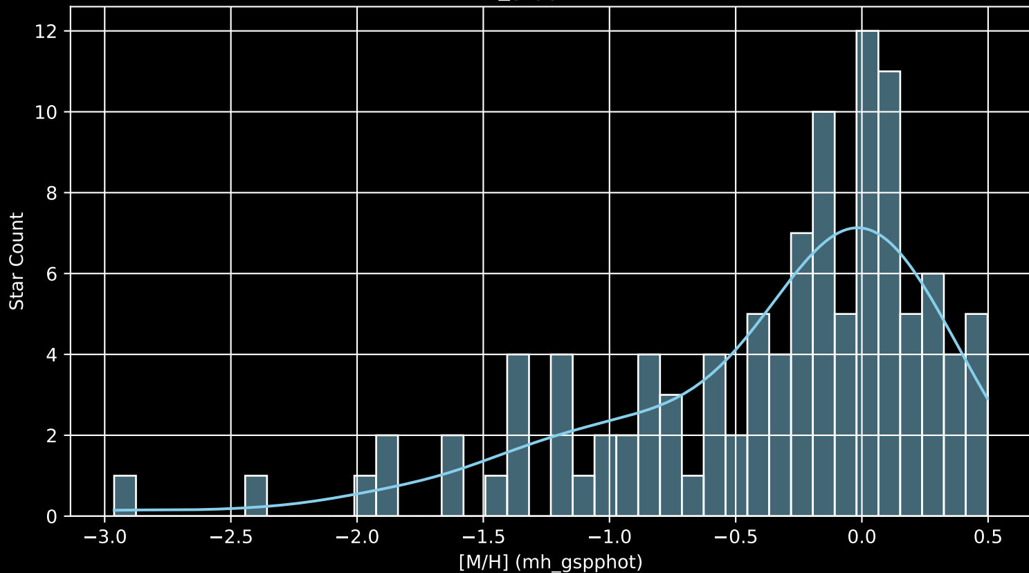
APOGEE DR17 Field: [345+00 [M/H] (mh_gspphot) (n= 109)
