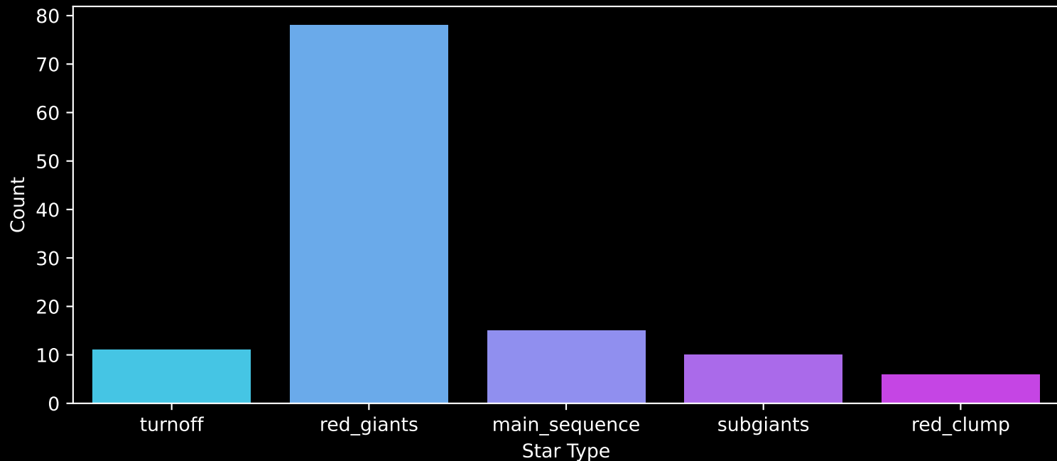
APOGEE DR17 Field: [345+00] Count plot of Star Type
