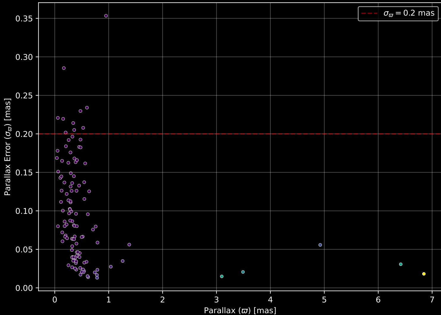
APOGEE DR17 Field: [345+00] Parallax Quality (n= 120)
