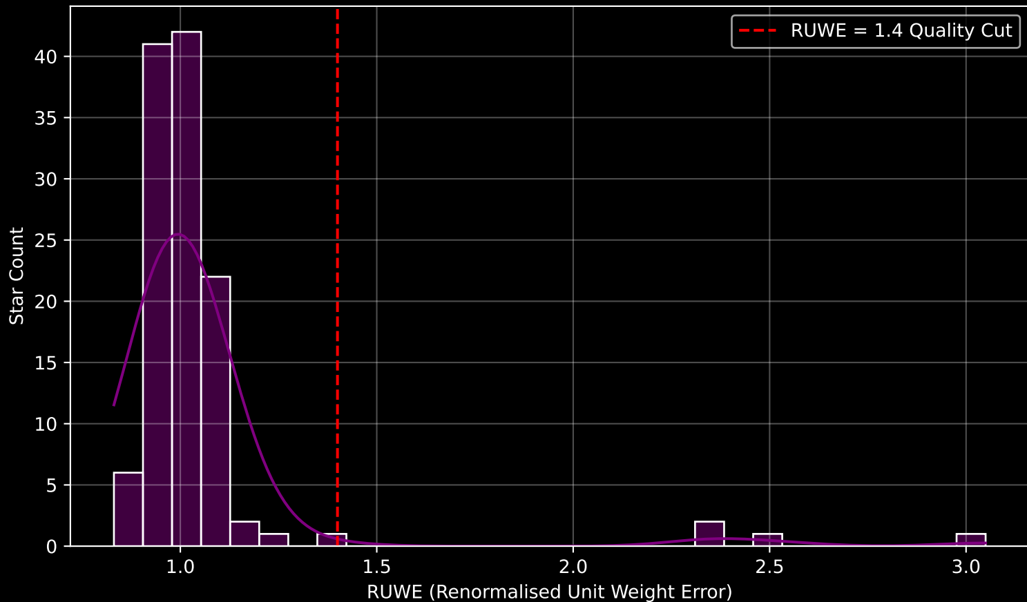
GAPOGEE DR17 Field [345+00] RUWE Distribution (n= 119)
